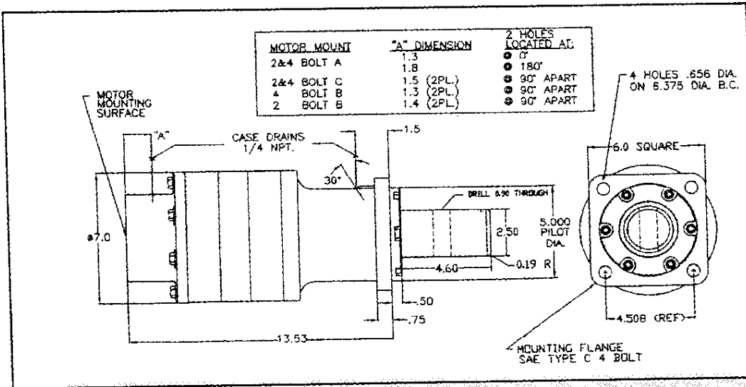
16DFF7 FRONT FLANGE
