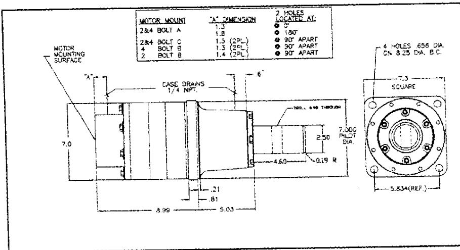
16DCF7 CENTER FLANGE
