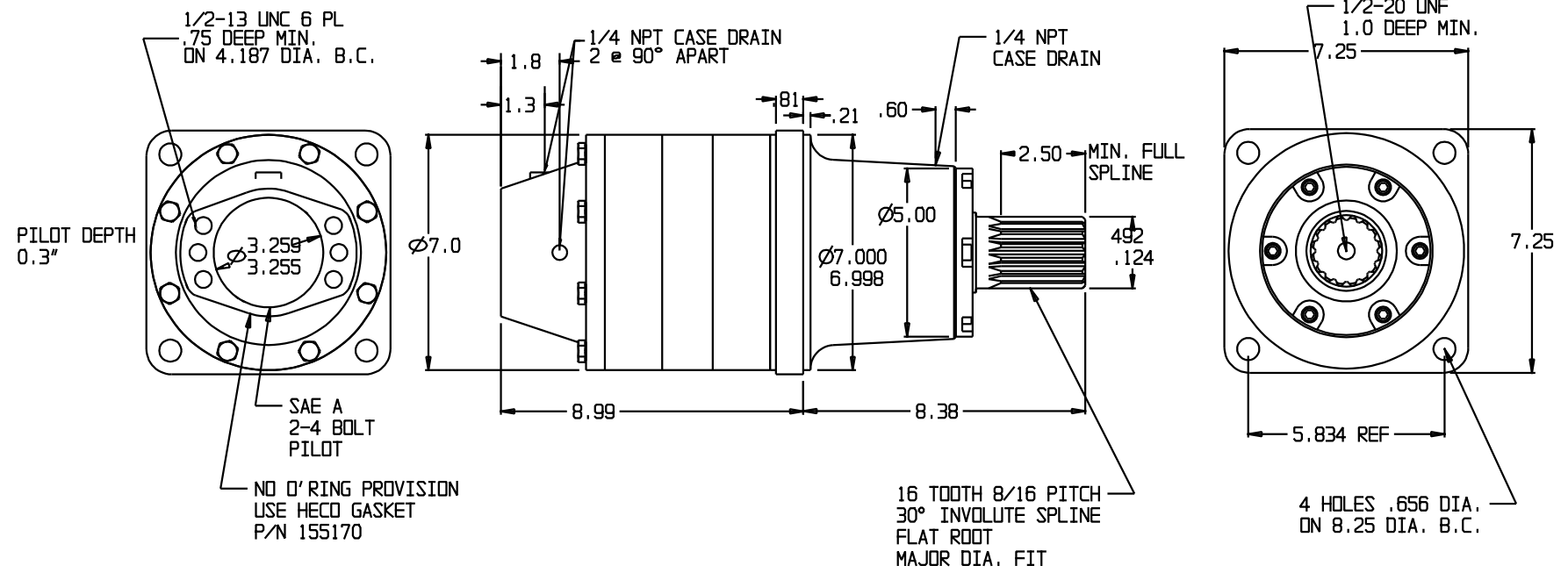
SUN GEARS- SUGGESTED MOTOR SHAFT LENGTHS
