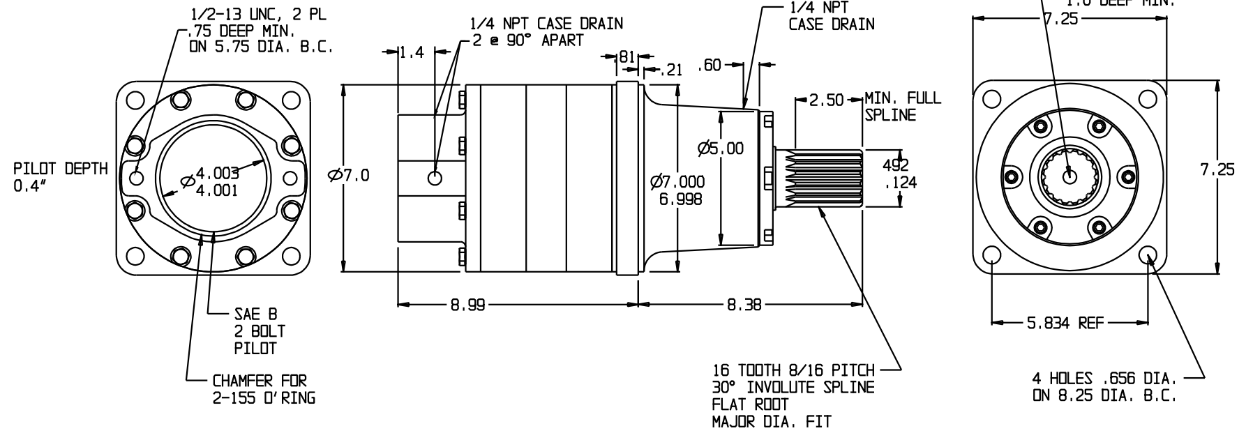
SUN GEARS- SUGGESTED MOTOR SHAFT LENGTHS
