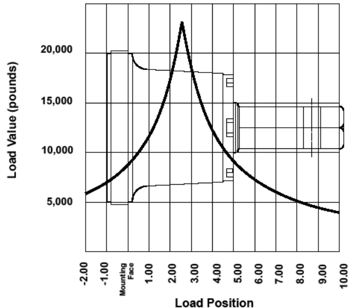
Shaft Load vs. Load Position 18,000,000 Revolution L 10 Life 85W-140 Gear Oil
